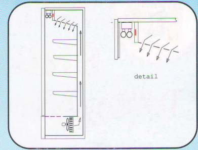
Supermarket Frozen Food Cabinets
