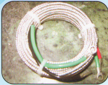
Single Cord Heater
